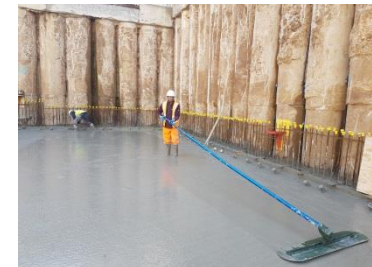
Casting of basement slab
